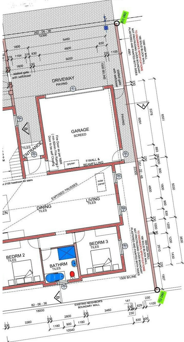
GROUND STOREY & SITE PLAN
