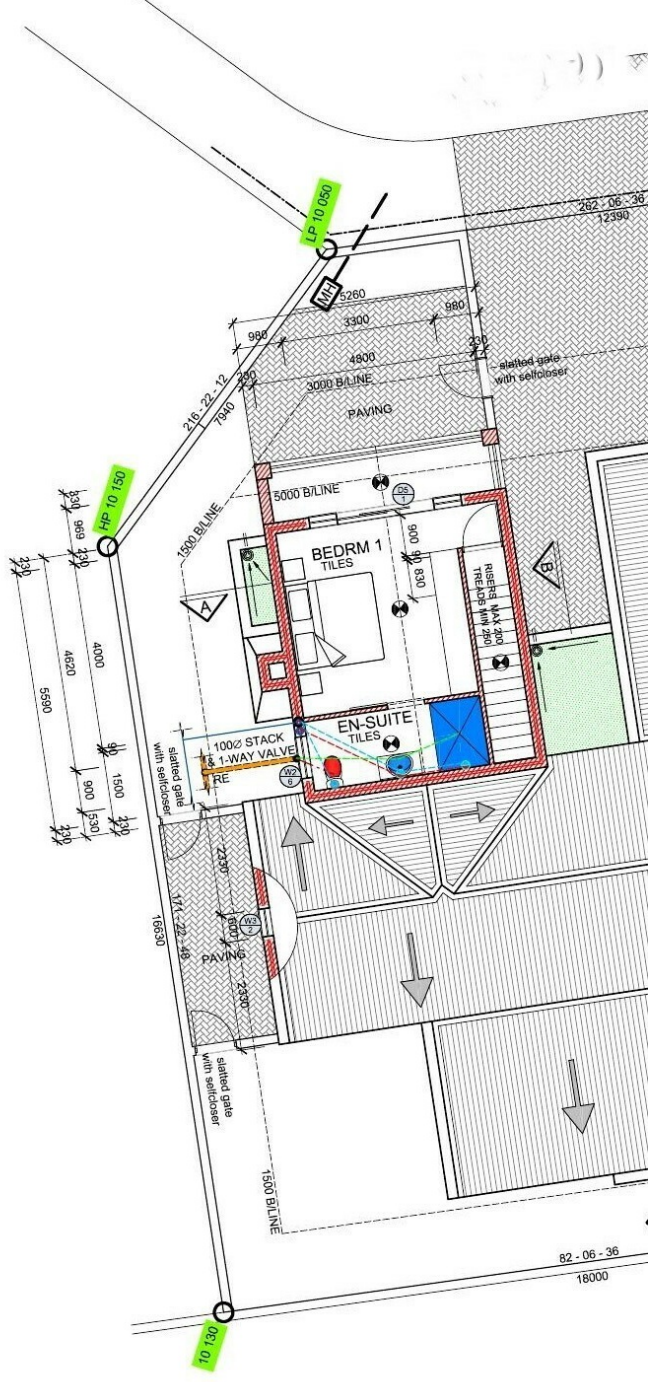
FIRST STOREY, SERVICE PLAN
